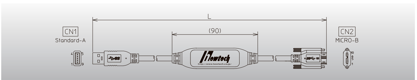
Example of a finished product : Standard-A to Micro-B(with Screw)
